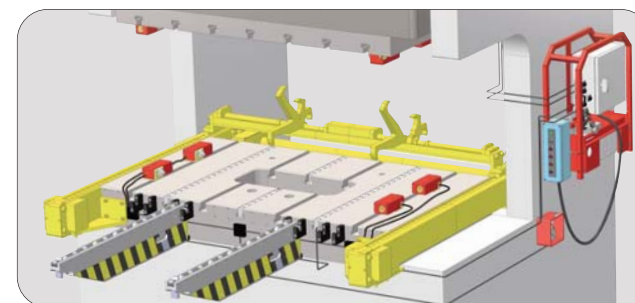
Press equipment for quick die change system
