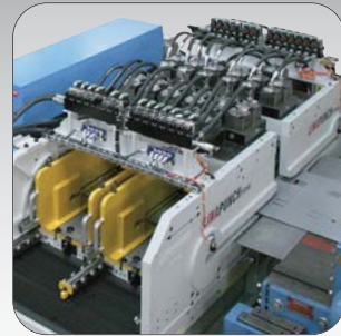
Linapunch® YT12 (hydraulic)
