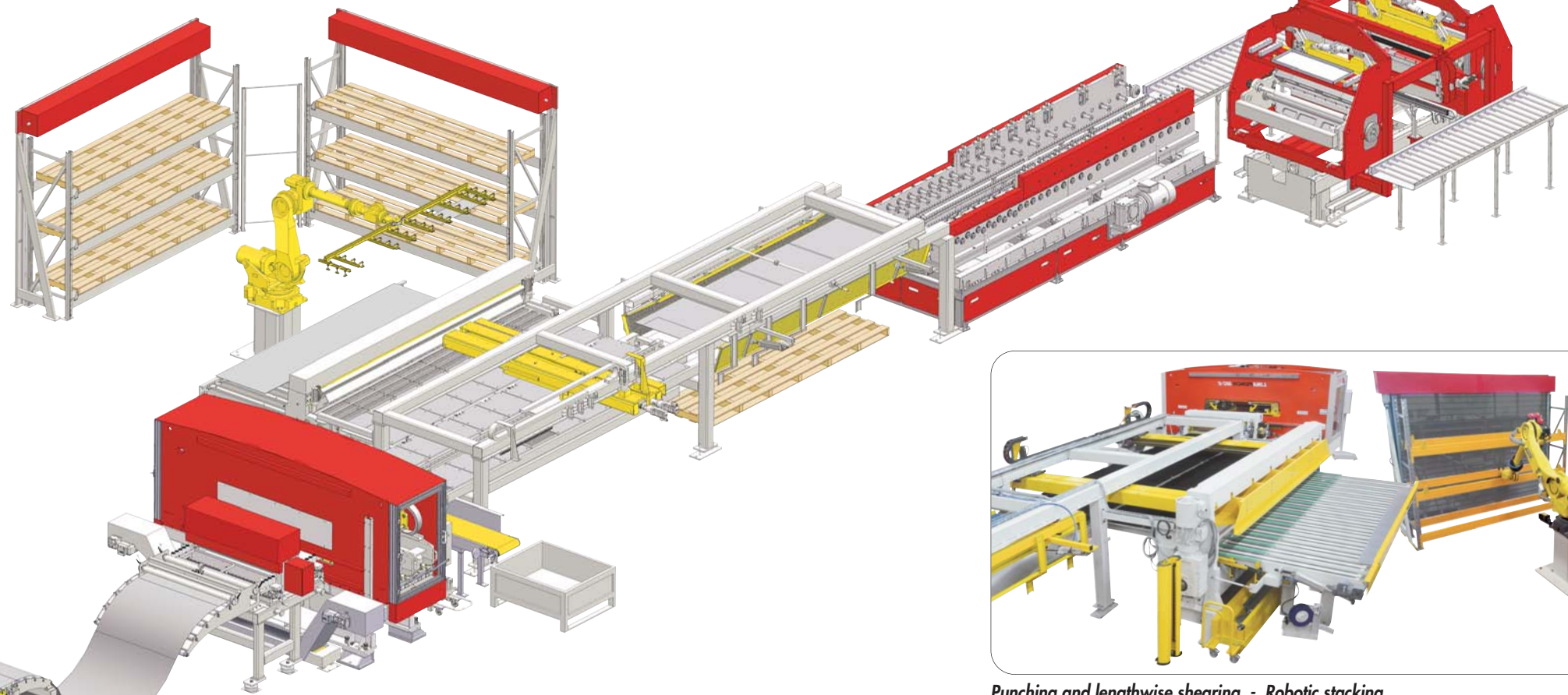
Punching and lengthwise shearing - Robotic stacking
